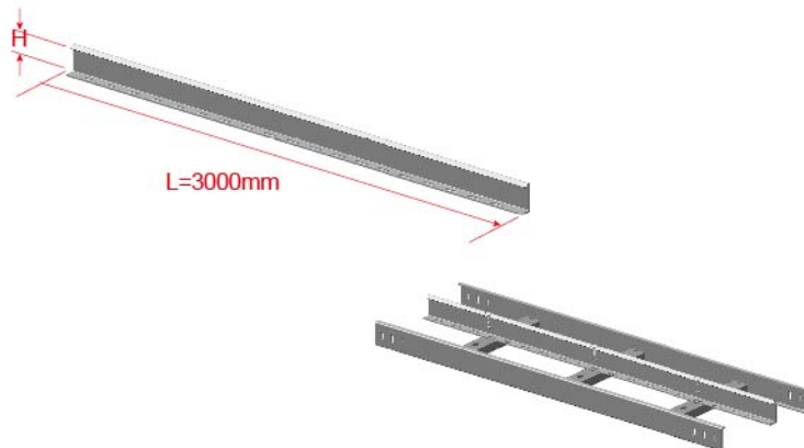
BL2-D Divider
