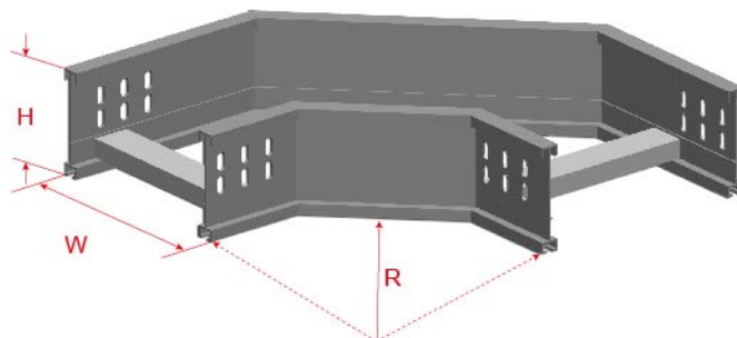
BL4/N20CA-E Elbow 90°
