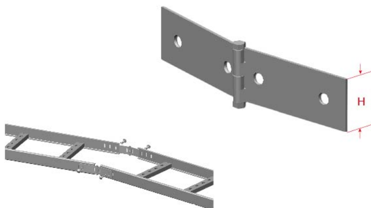
BL1/2/3-HAC N12B/16A/20B/20C-HAC Horizontal Adjust Coupler
