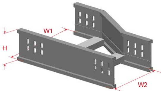
BL4/N20CA-RR Right Hand Reducer
