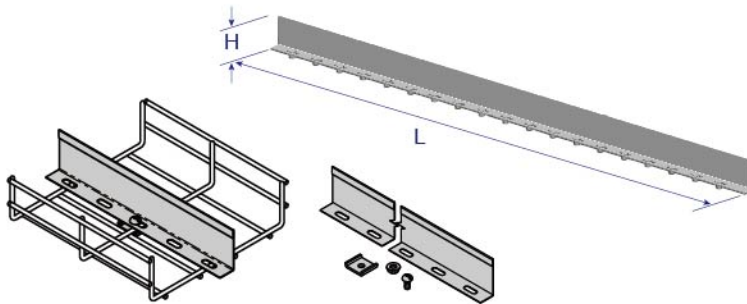
BM*-B Barriers
