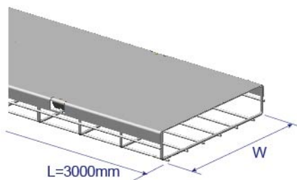
BM-C Cover
